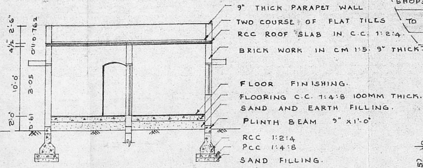
SECTION R-S
